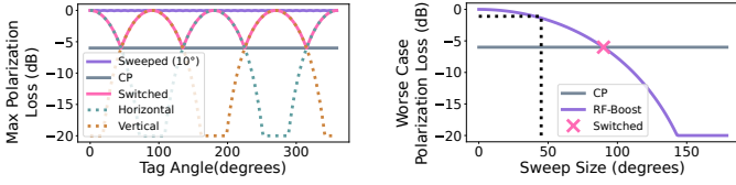
(a) Polarization Loss vs Tag Angle (b) Worst-Case Loss vs Sweep Size Fig. 3: Polarization Loss Simulations. a) Simulation results of polarization loss when sweeping with 10° granularity (purple), switched (pink), horizontal (green), vertical (brown), and CP (gray). b) Simulation results of worst-case polarization loss vs sweep size (purple) compared to CP (gray) and switched polarization (pink x). Dotted lines denote loss at 45° granularity.
